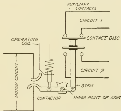
Fig. 62. Diagram of Sprague-General Electric Interlock
